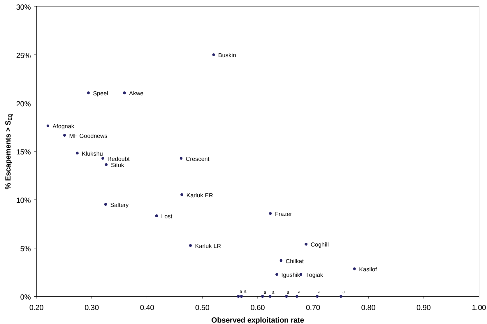
Figure 9. —Percentage of escapements greater than carrying capacity ( S_{EQ} ) plotted against the observed exploitation rate for 29 sockeye salmon stocks with a reliable estimate of S_{EQ} (Italo stock not shown).
