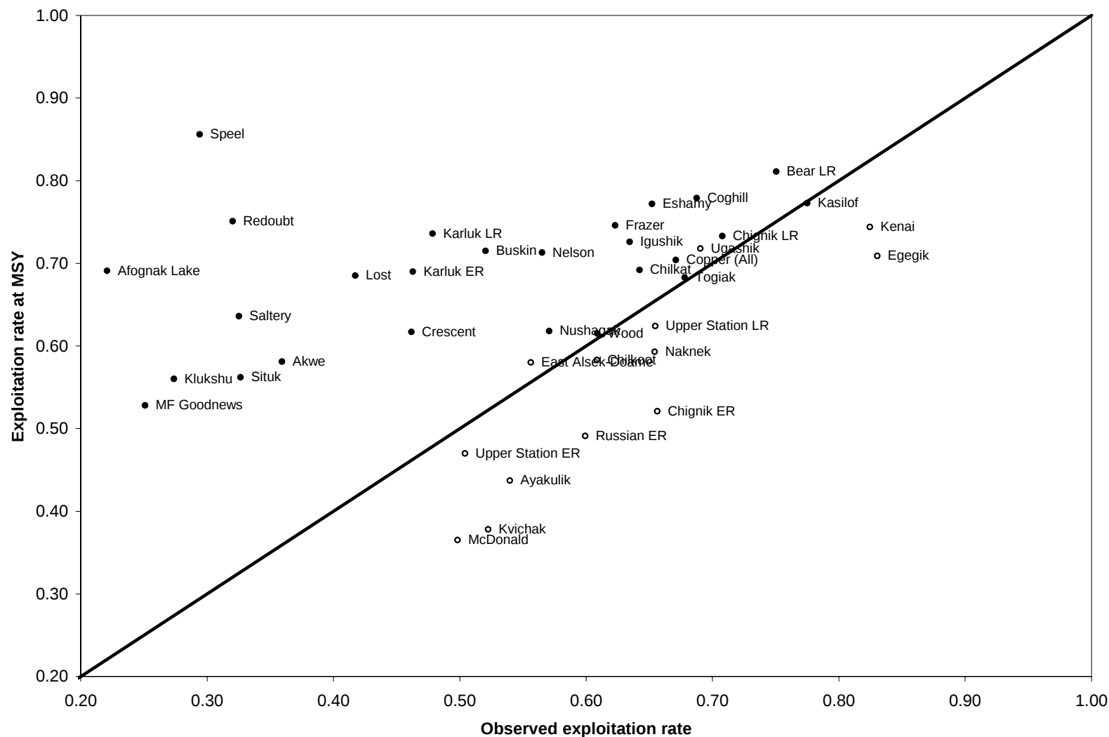
Figure 8. —Estimated exploitation rate at MSY determined from \ln \alpha' plotted against the observed exploitation rate for 40 Alaskan sockeye stocks (Italo stock not visible in this plot). Open circles designate stocks that do not have a reliable estimate of carrying capacity (NPCV of S_{EQ} > 0.250 ) and closed circles designate stocks that do have a reliable estimate of carrying capacity (NPCV of S_{EQ} \leq 0.250 ).
